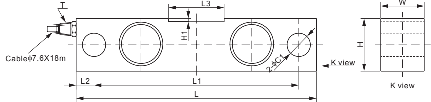
Capacity: 75Klb
