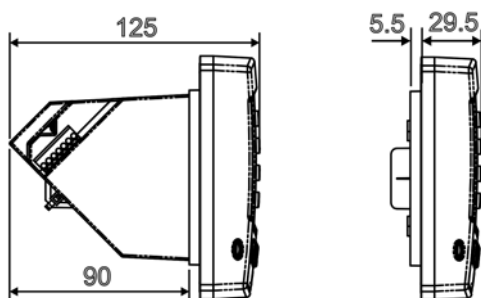
Side View with Boot and Stand
