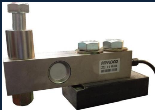
Shows an ASCI Weigh Mount with a 5t 563YH Load Cell
